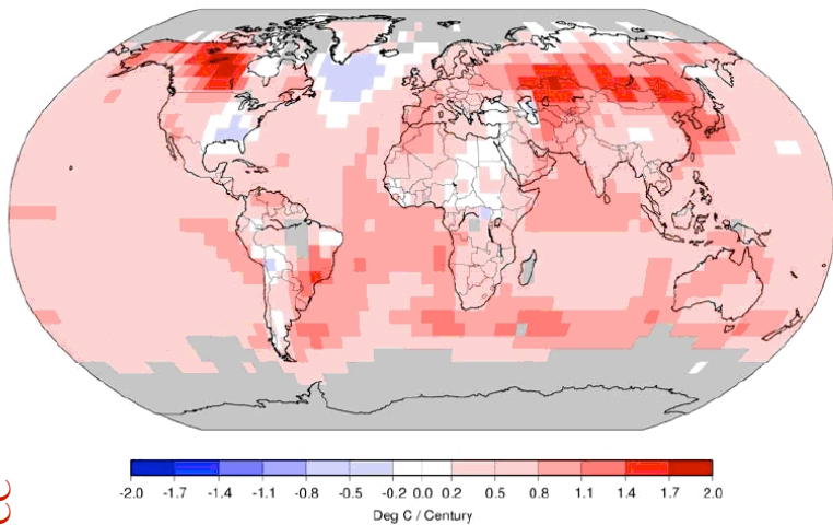
Trend in Annual TMEAN, 1901 to 2004
